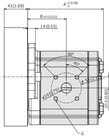
SAE-B Pressure Side, Side View
