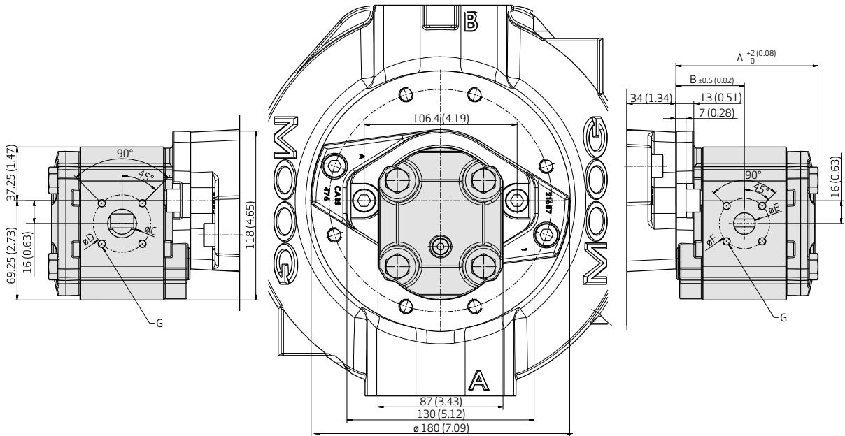
SAE-A Suction Side, Side View
