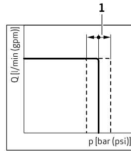
1 Screw adjustment
